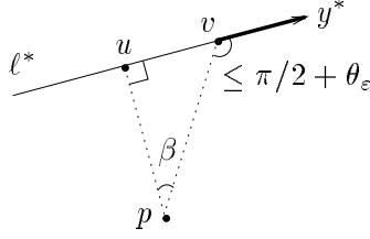
Figure 1: The plane containing the line \ell^* and the point p .
