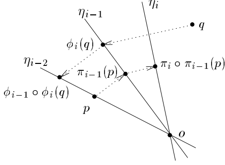
Figure 1: The projections \phi_i and \pi_i .
