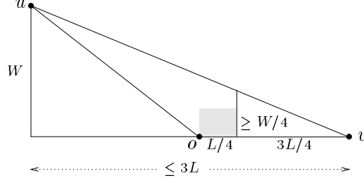
Figure 2: \triangle ovu contains a box of length L/4 and width W/4 . (The easier case when \angle uov < \pi/2 is omitted.)
