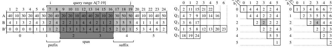
■ Figure 1 The array has size n = 24 (of which \Delta = 5 are distinct), partitioned into s = 6 blocks of size t = 4 . The query range is A[i:j] = A[7:19] , for which the unique mode is 20, occurring with frequency 5. The corresponding mode of B[i:j] is 2. The query range is partitioned into the prefix B[7:8] , the span B[9:16] , and the suffix B[17:19] . The span covers blocks b_i = 2 to b_j = 3 , for which the corresponding mode is S[2,3] = 2 , occurring with frequency S'[2,3] = 4 .
