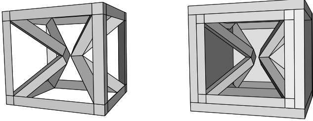
Figure 2: (Left) Base polyhedron with genus 11. (Right) Polyhedron with genus 6 after adding a thin box layer on the outside of all but one face.
