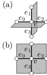
Figure 5: Possible faces around a degree-4 vertex.
