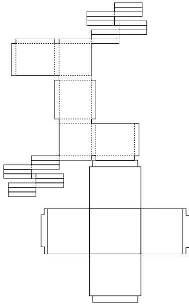
Figure 4: Net for Figure 2.
