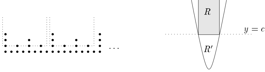
Figure 1: (Left) Proof of Lemma 4.1: the point set P and two level-1 rectangles (with b = 2 and k = 4 ). (Right) Proof of Theorem 4.2: the rectangle R = [a, b) \times [c, \infty) and the parabolic range R' = \{(x, y) : y - c \geq m(x - a)(x - b)\} . As m \rightarrow \infty , R' approaches the slab [a, b) \times \mathbf{R} .
